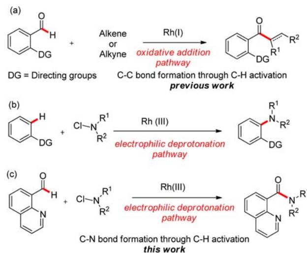
Scheme 1. Coupling Reactions through C–H Activation
